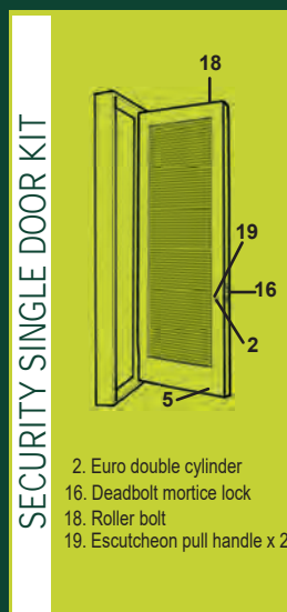
SECURITY SINGLE DOOR KIT
